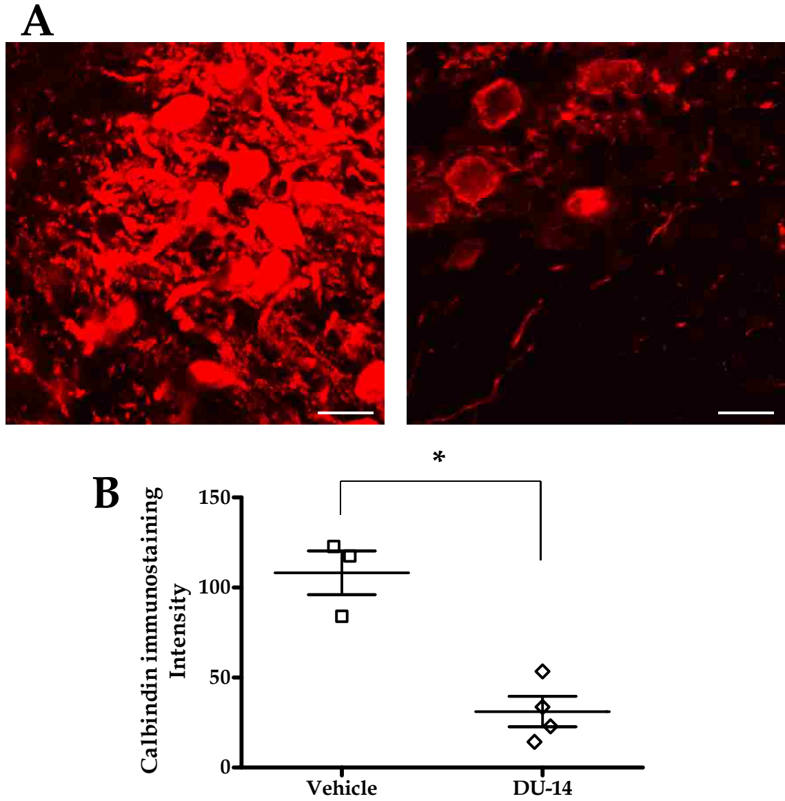
Figure 5.2. Prolonged inhibition (DIV12-28) of steroid sulfatases decreases PC viability.
