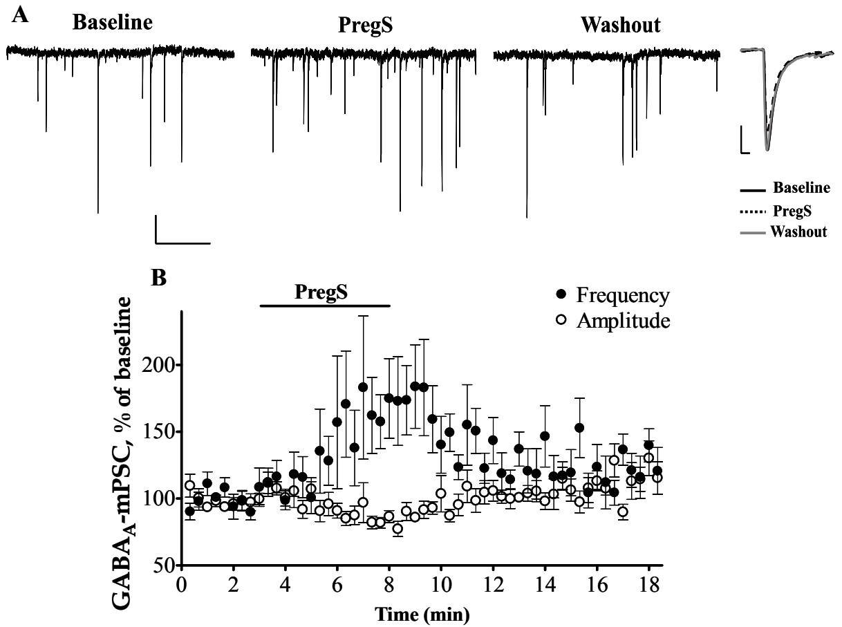
Figure 3.7. PregS (25 \mu M) increases the frequency of GABA A -mPSCs in PCs from neonatal rats
